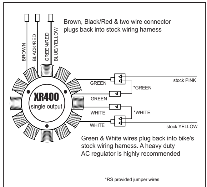
Diagram 4: Single output of 200 watts
